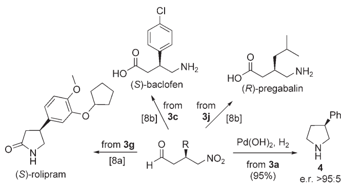
Scheme 2. Synthetic applications of \gamma -nitroaldehydes.
