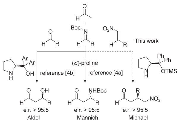
Scheme 1. Acetaldehyde as a nucleophile in enamine catalysis. TMS = trimethylsilyl.
